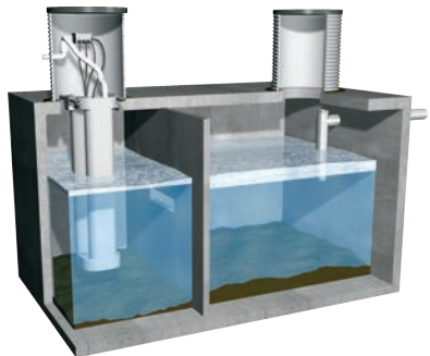
Concrete Tank
